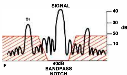
Figure 3. A bandpass filter removes unwanted signals at frequencies less than the low cut-off and greater than the high cut-off frequency.
